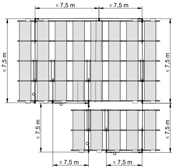
OUTSIDE CORNER
